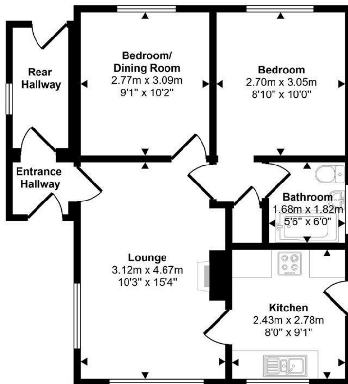
Floorplan
